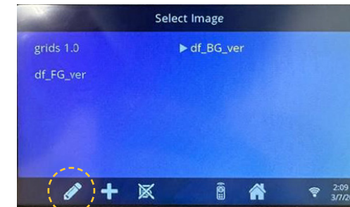
17.20 Edit Image
