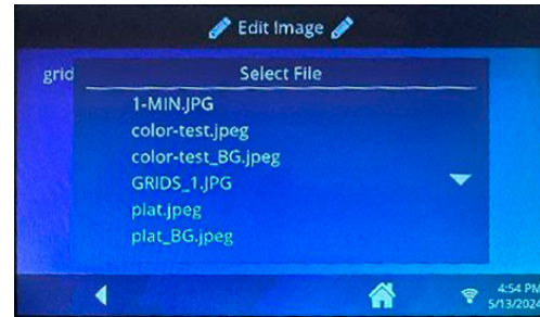
17.17 Select Image
