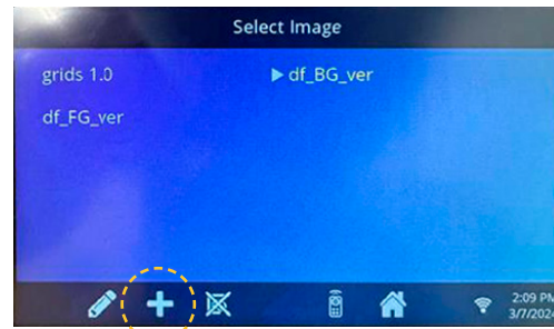
17.15 Add Image
