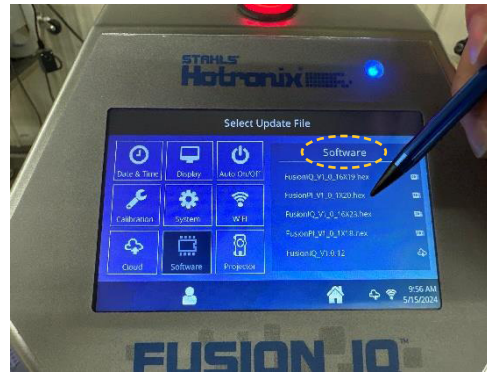
21.6 Software List
