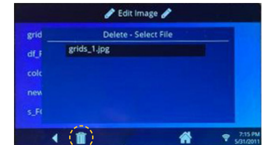
17.23 Trash Icon
